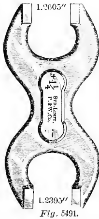
M. C. B. STANDARD LIMIT GAUGE. For 1 1/4 in. round iron. See Dictionary for table of other standard Limit gauges.
